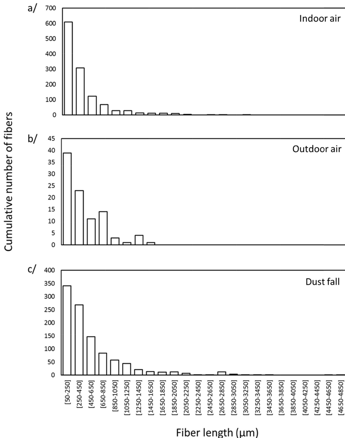
Fig. 2. Cumulative number of fibers observed in each size range between 50 and 4850 μm in various samples, a/indoor air, b/outdoor air, c/dust fall.
